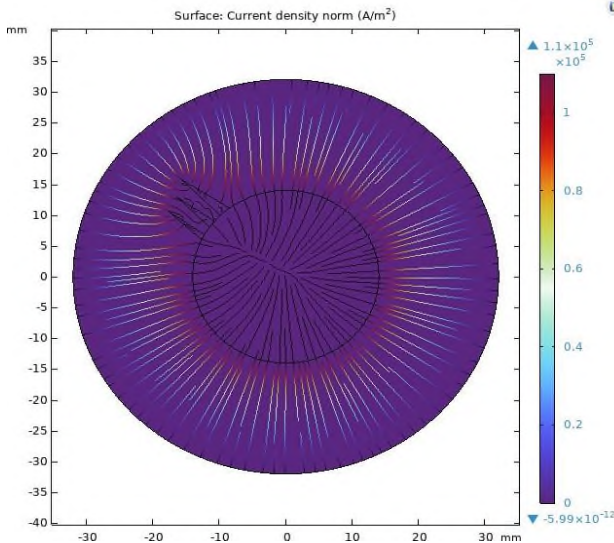
Figure 8. Distribution of current density in the branches of water tree
