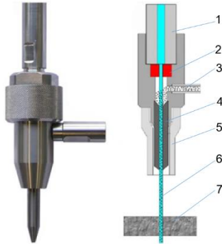
Figure 1. Hydroabrasive cutting diagram
