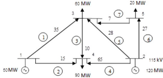
Fig. 9. Scheme for the calculating addressed transmitting of power
