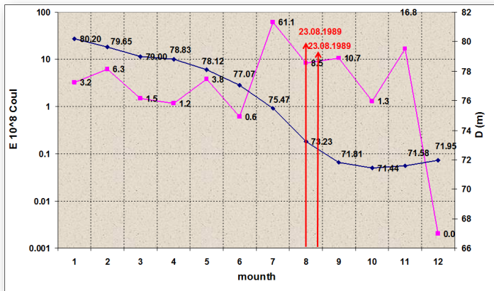
Figure. 10. Schedule of activation of landslide processes as a result of energy released during earthquakes caused by water changes in Mingachevir water basin during 1989
