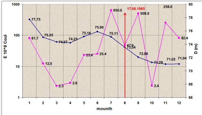
Figure. 9. Schedule of activation of landslide processes as a result of energy released during earthquakes caused by water changes in Mingachevir water basin during 1985
