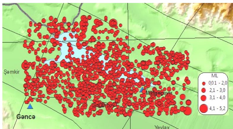
Figure. 4. Map of epicenters in the territory of Mingachevir for 1954-2017 (N = 1290)
