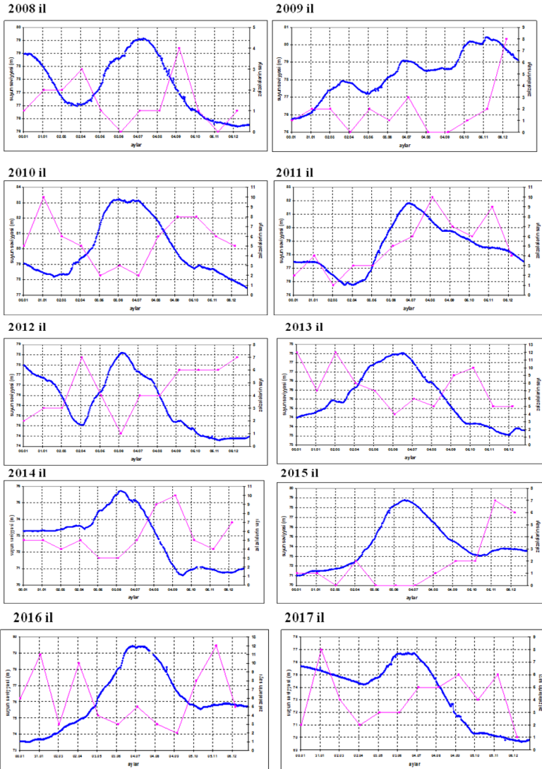
Figure 6. Histogram of water level and number of earthquakes in the reservoir 4
