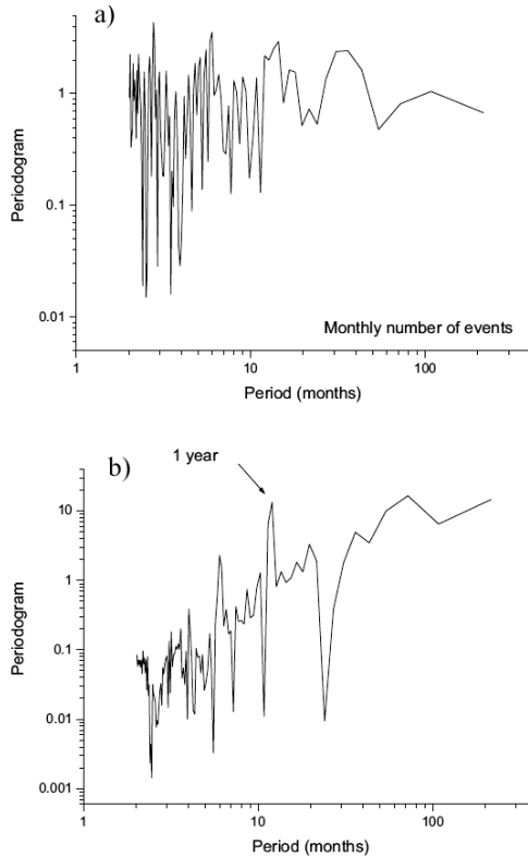
Figure 8. Correlogram of the monthly periodogram of the number of earthquakes (a) and water level (b)
