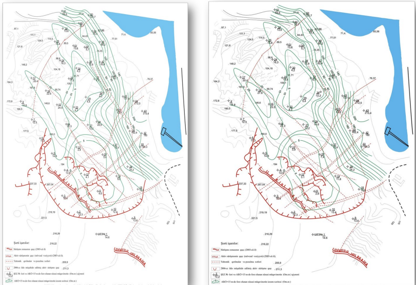
Figure. 1. Map of monitoring results of SEZ ( AB / 2 = 15 \text{ m} ) in the dam part of Mingachevir reservoir for October and December 2006 (compiled by: R.F. Huseynov)
