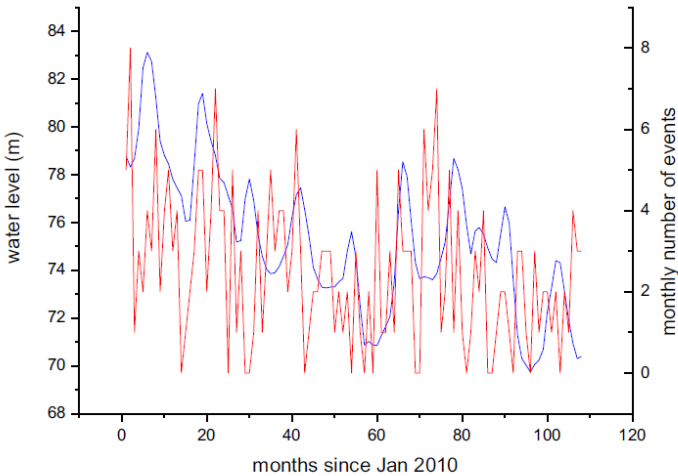
Figure. 7. Graph of change of water level and average values of earthquakes by months (time magnitude \geq 1.6 )
