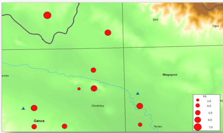
Figure 3. Map of epicenters of Mingachevir region and adjacent territories for 1900-1954
