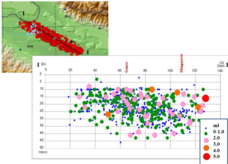
Figure. 5. Seismological section of I-I profile of Mingachevir water basin area (2003-2017)
