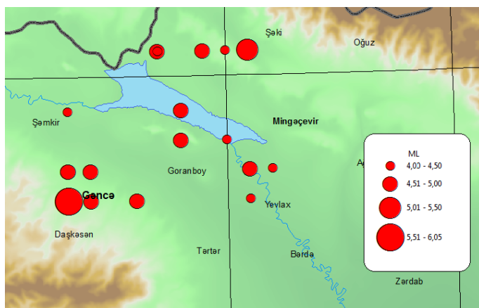
Figure. 2. Map of epicenters of earthquakes with magnitude 4.0 near Mingachevir water basin during 1900-2017
